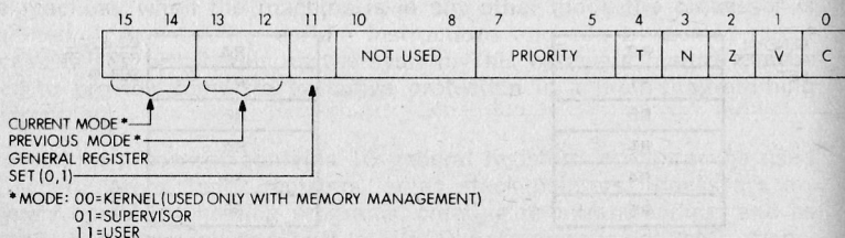
Figure 10-4 Processor Status Word
