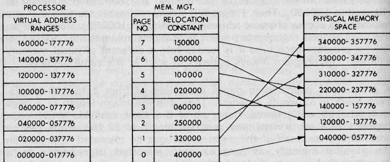
Figure 9-3 Relocation of a 32K Word Program into 124K Word Physical Memory
