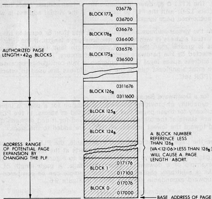
Figure 9-7 Example of a Downward Expandable Page
