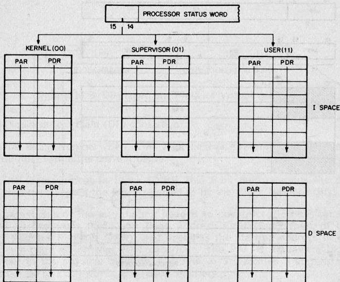
Figure 11-5 Active Page Registers
