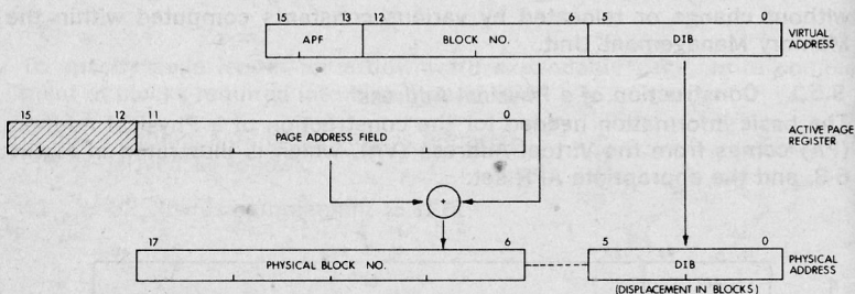
Figure 9-10 Construction of a Physical Address
