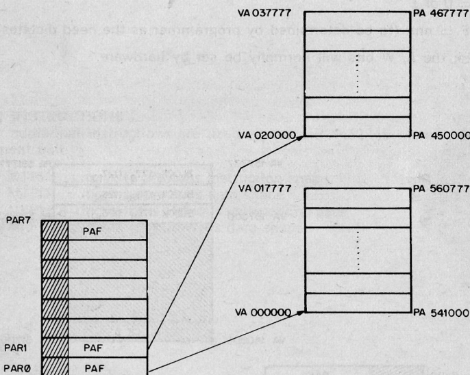
Figure 11-12 Non-Consecutive Memory Pages
