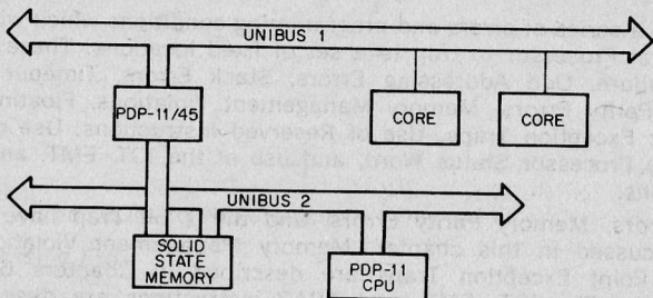
Figure 10-6 Multiprocessor Use of the Second UNIBUS
