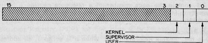
Figure 11-10 Format of Status Register #3 (SR3)
