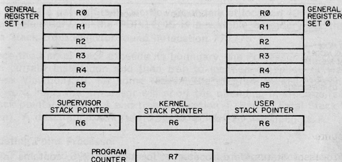
Figure 10-3 The General Registers
