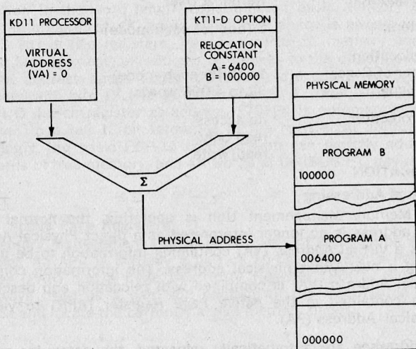
Figure 9-2 Simplified Memory Relocation Example
