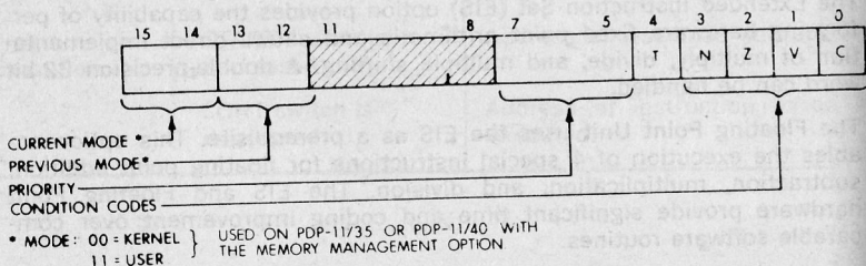
Figure 8-1 Processor Status Word
