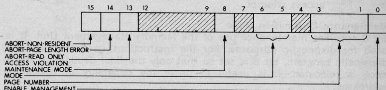
Figure 9-11 Format of Status Register #0 (SR0)
