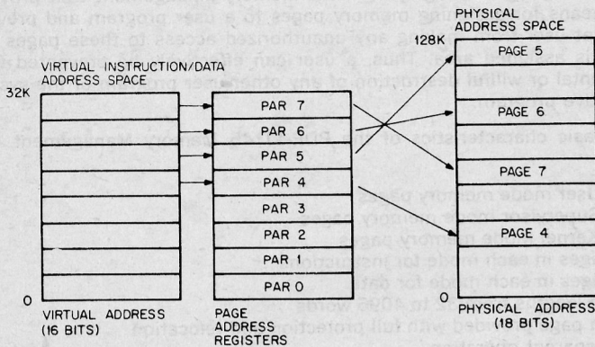
Figure 11-1 Virtual Address Mapping into Physical Address
